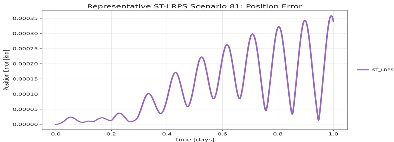
(b) Representative Case: Scenario #81 | h_p = 295 km, i = 103 deg | RMS = 0.16 m, max = 0.36 m
