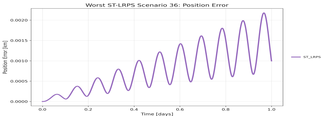
(c) Worst Case: Scenario #36 | h_p = 226 km, i = 167 deg | RMS = 0.96 m, max = 2.18 m
