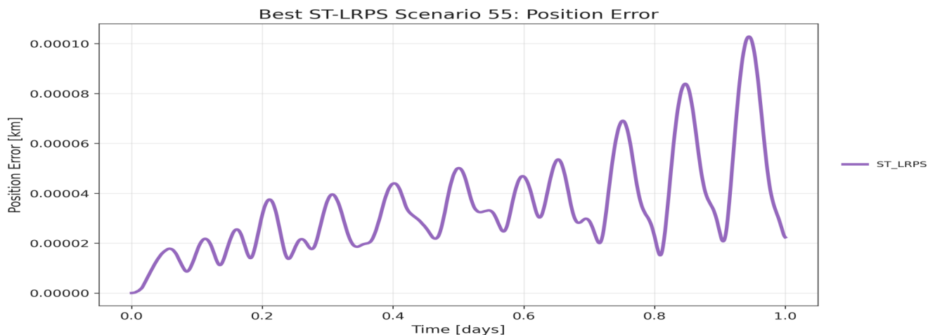
(a) Best Case: Scenario #55 | h_p = 347 km, i = 125 deg | RMS = 0.04 m, max = 0.10 m
